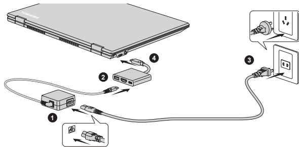
Figure 4-8 Connecting the AC adaptor via USB Type-C™ adapter
